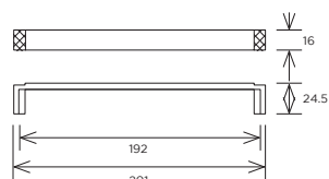
Dunston D-Handle
