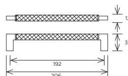
Didsbury D-Handle
