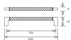
Didsbury D-Handle
