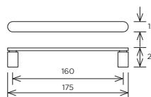
Lloyd D-Handle
