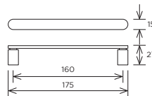
Lloyd D-Handle
